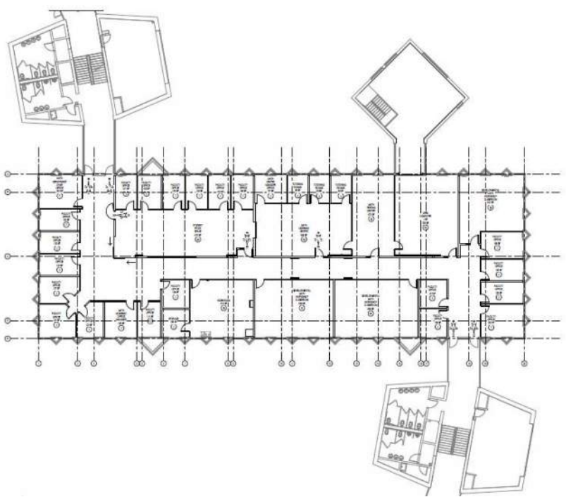
Building B Second Floor Plan
