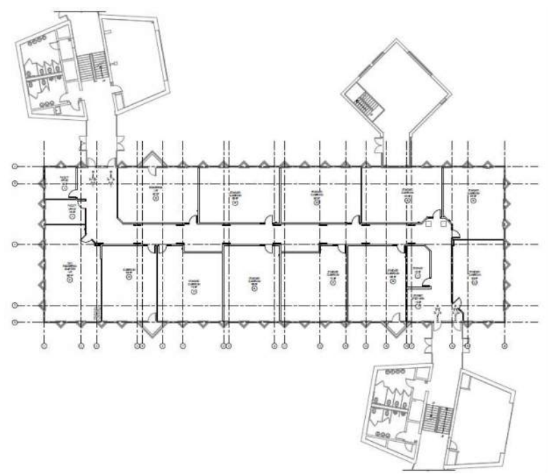
Building B First Floor Plan
